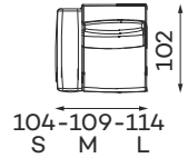
2,5-SEATER WITH ARMREST
