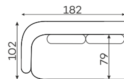
2-SEATER WITH ARMREST.
